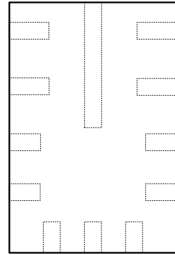
Figure 1. 12-Lead QFN 2mm×3mm
