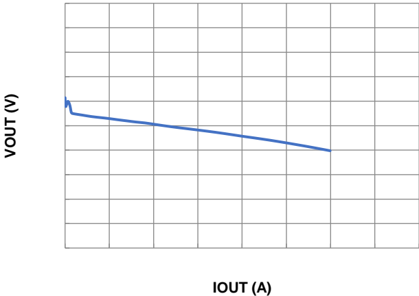
Figure 3. Load Regulation
